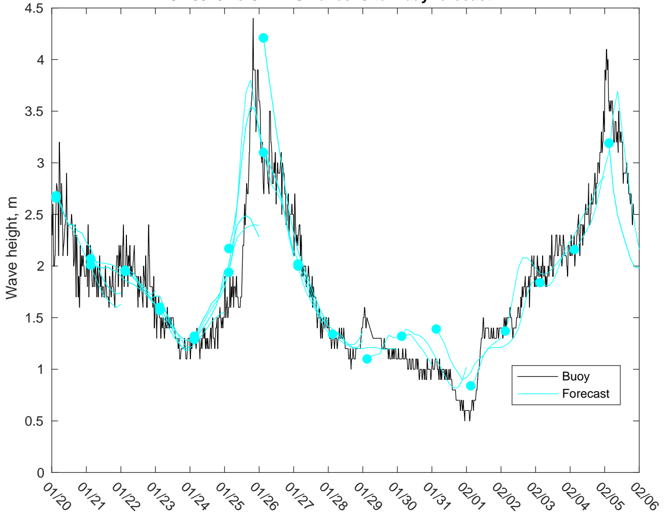
NDBC 46028 vs CMEMSWaves: 5 to 7 day forecast
