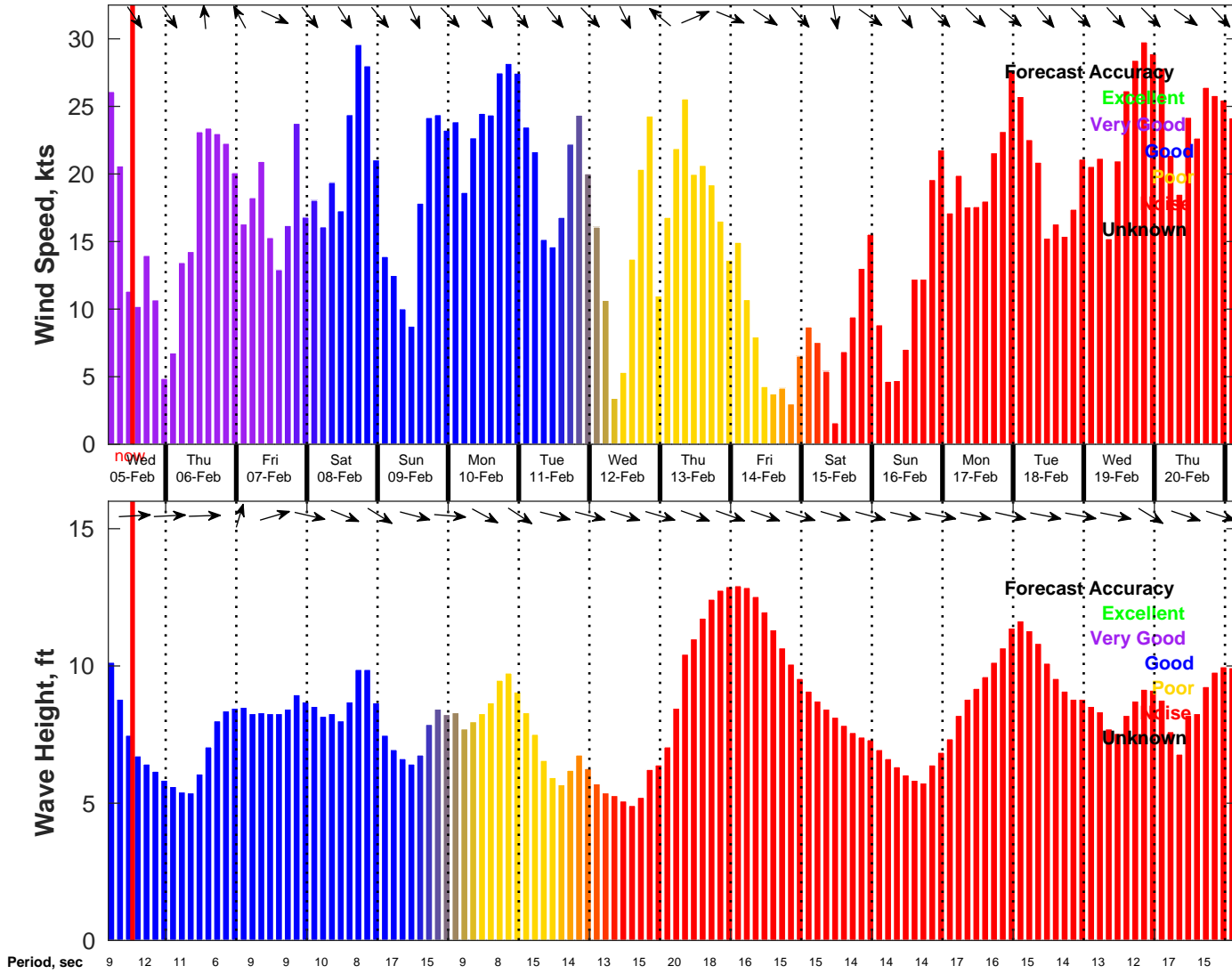
Wind & Wave Forecast for NDBC 46028 from 05-Feb-2025 04:00:00 to 21-Feb-2025 04:00:00
