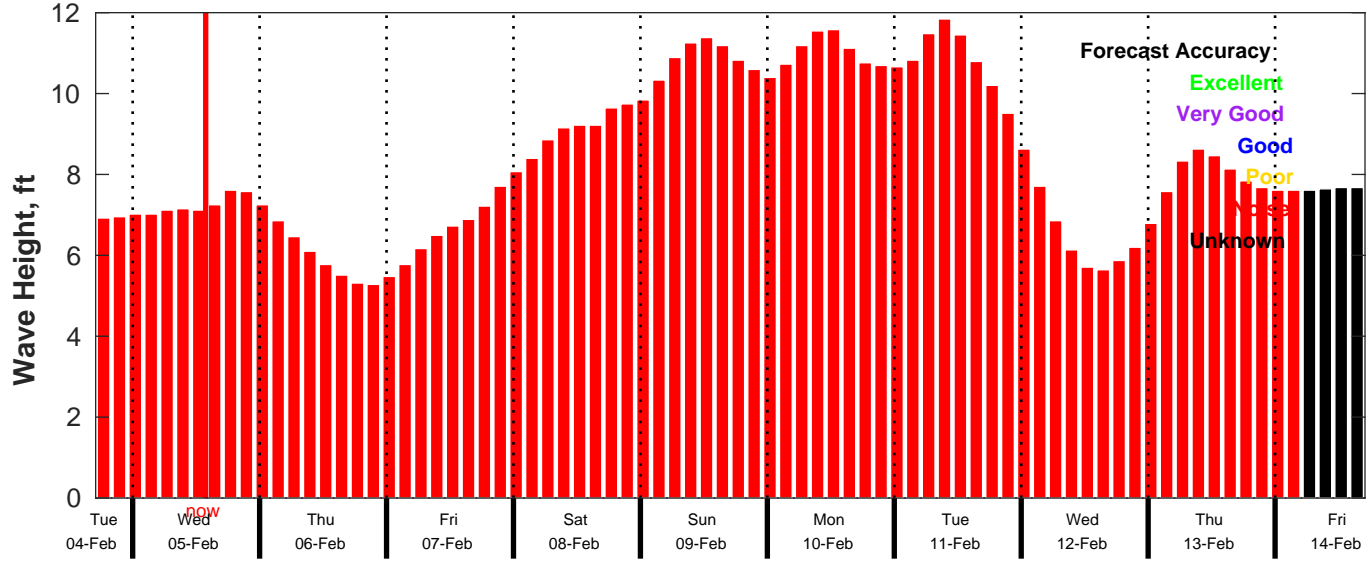
CMEMS Wave Forecast for NDBC 46053 from 04-Feb-2025 17:00:00 to 14-Feb-2025 17:00:00
