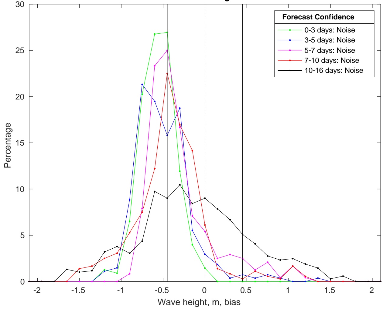
NDBC 46054 vs GFSWaves Bias Histogram: 05-Feb-2025
