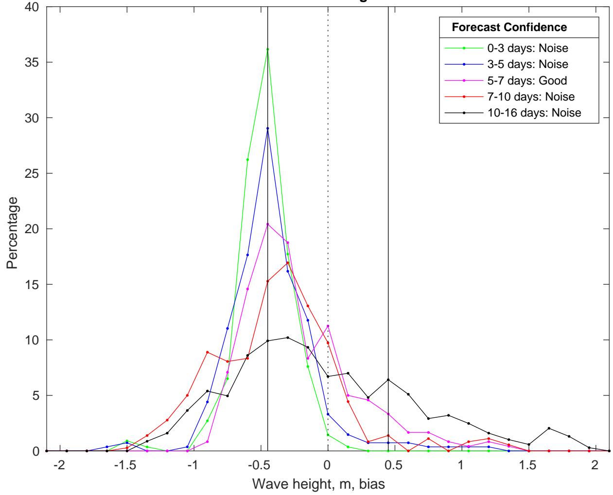
NDBC 46069 vs GFSWaves Bias Histogram: 05-Feb-2025
