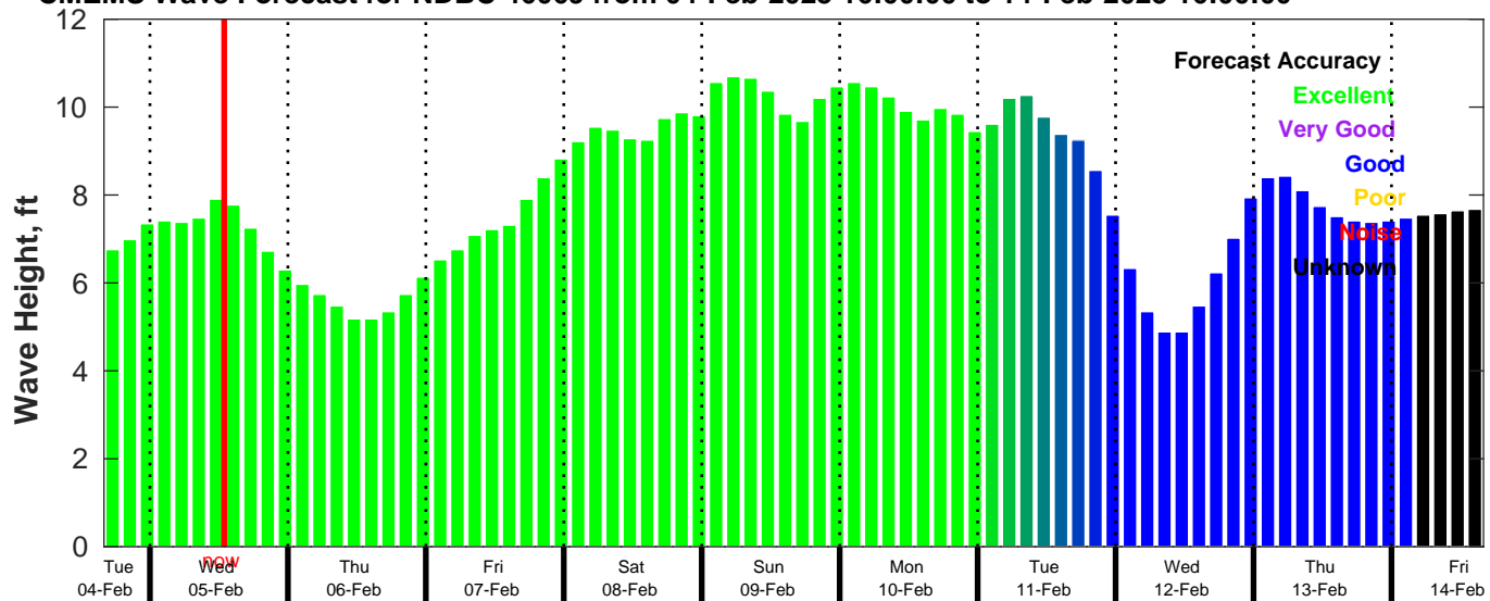
CMEMS Wave Forecast for NDBC 46069 from 04-Feb-2025 16:00:00 to 14-Feb-2025 16:00:00
