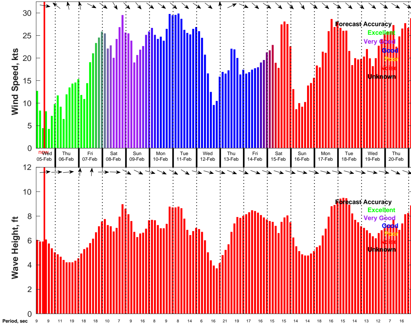
Wind & Wave Forecast for NDBC 46069 from 05-Feb-2025 04:00:00 to 21-Feb-2025 04:00:00
