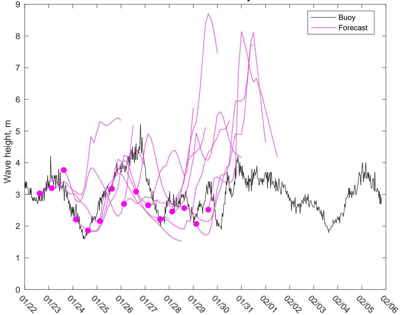
NDBC 46246 vs GFSWaves: 7 to 10 day forecast
