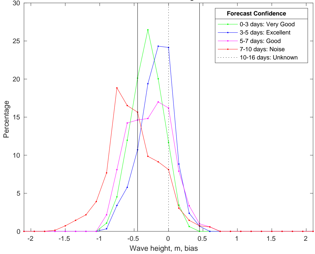
NDBC 52213 vs CMEMSWaves Bias Histogram: 05-Feb-2025
