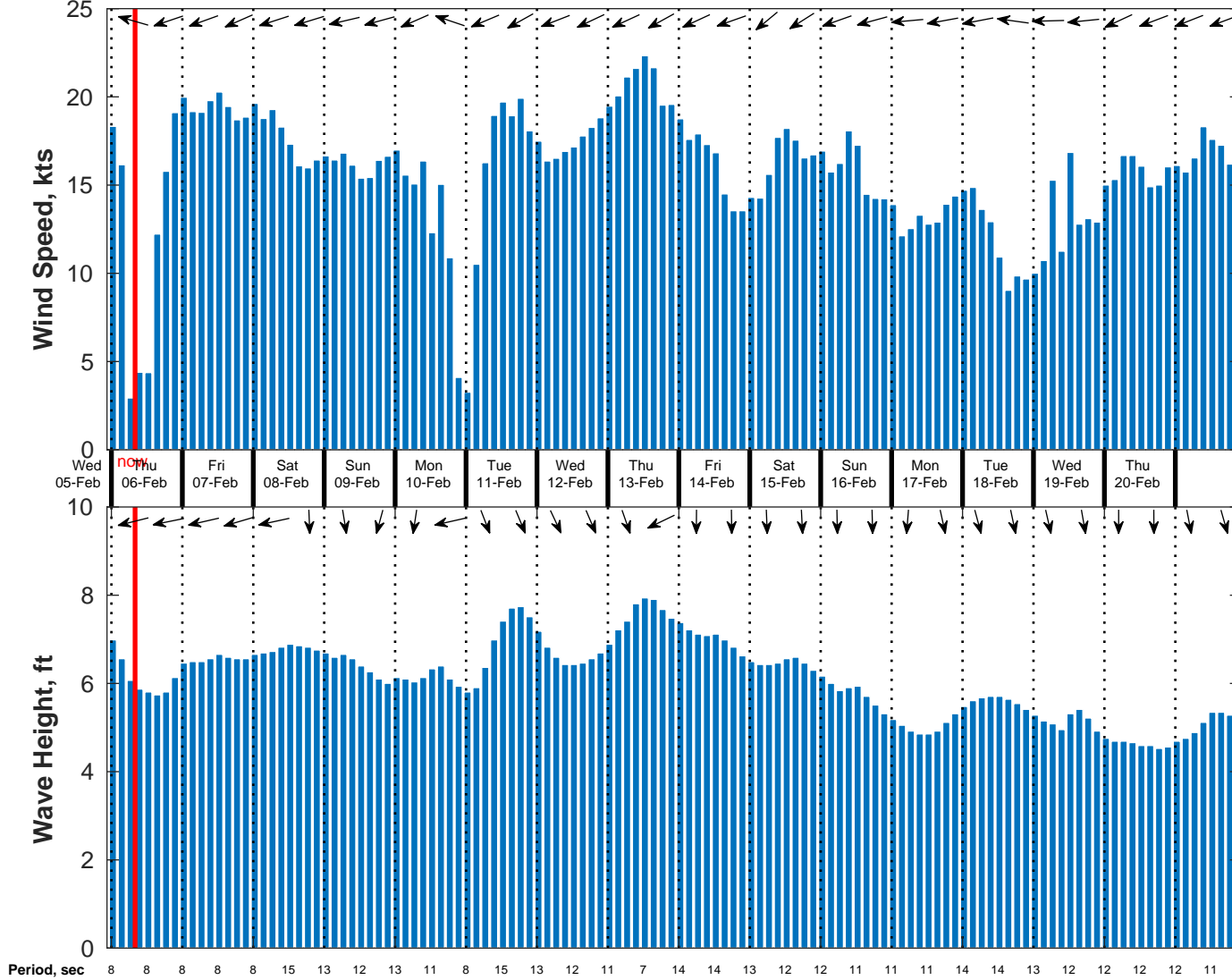
Wind & Wave Forecast for NDBC 52213 from 05-Feb-2025 23:00:00 to 21-Feb-2025 23:00:00
