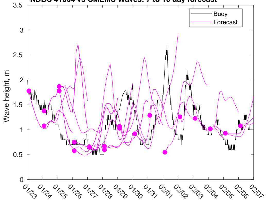
NDBC 41004 vs CMEMS Waves: 7 to 10 day forecast
