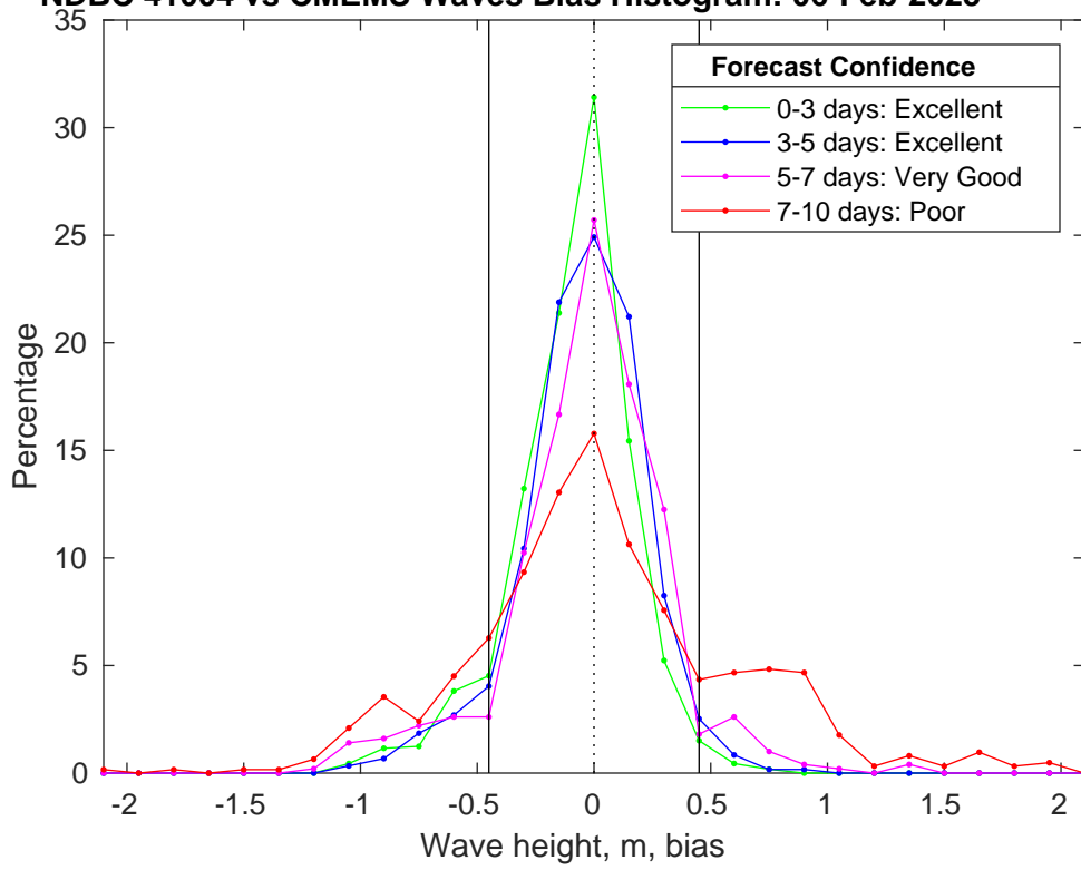
NDBC 41004 vs CMEMS Waves Bias Histogram: 06-Feb-2025
