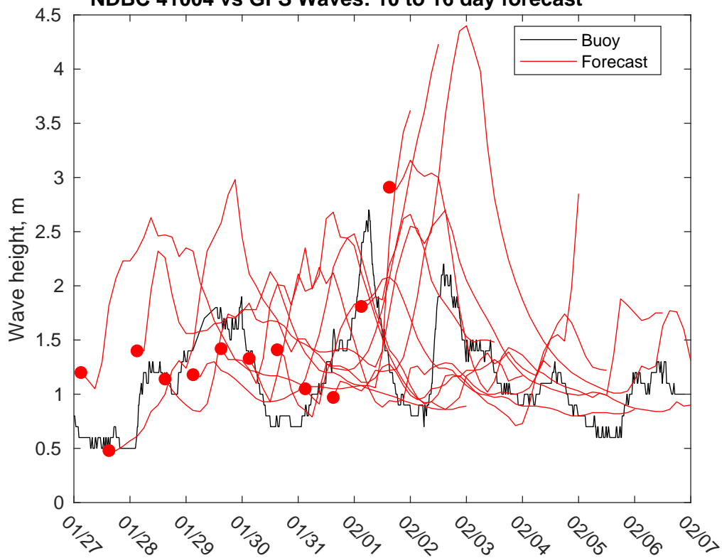
NDBC 41004 vs GFS Waves: 10 to 16 day forecast
