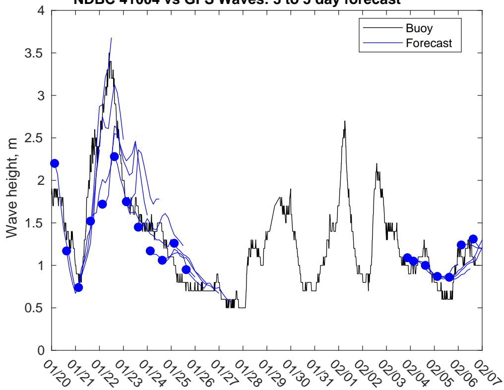
NDBC 41004 vs GFS Waves: 3 to 5 day forecast
