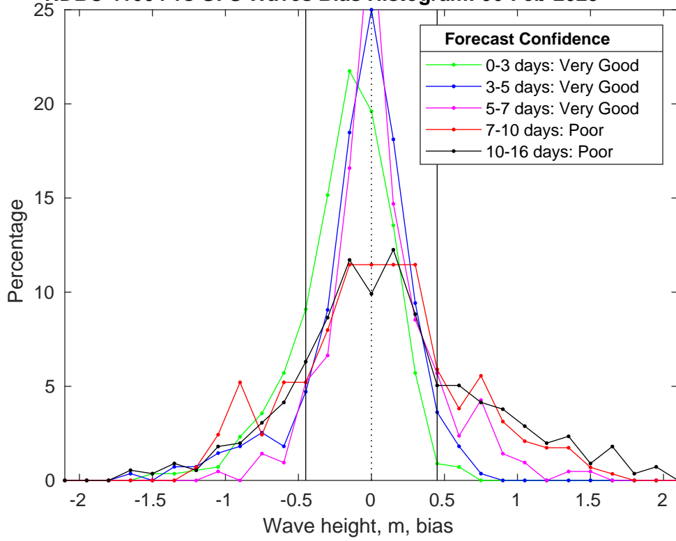
NDBC 41004 vs GFS Waves Bias Histogram: 06-Feb-2025
