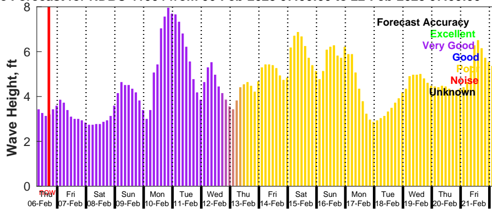
GFS Wave Forecast for NDBC 41004 from 06-Feb-2025 07:00:00 to 22-Feb-2025 07:00:00
