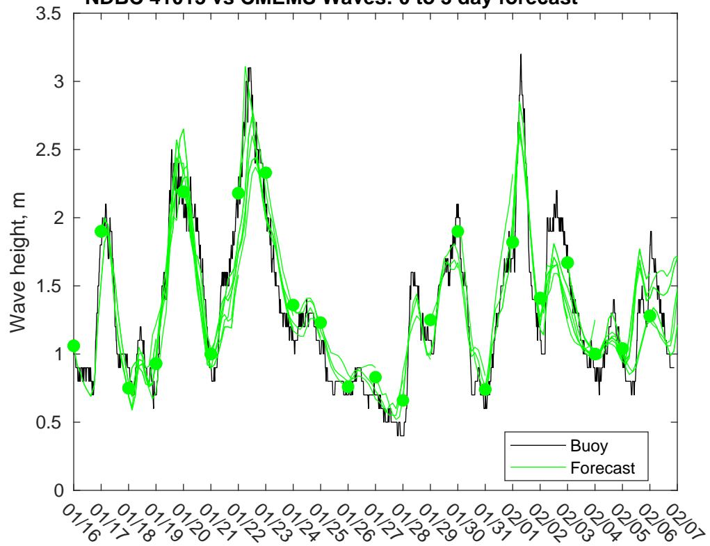
NDBC 41013 vs CMEMS Waves: 0 to 3 day forecast
