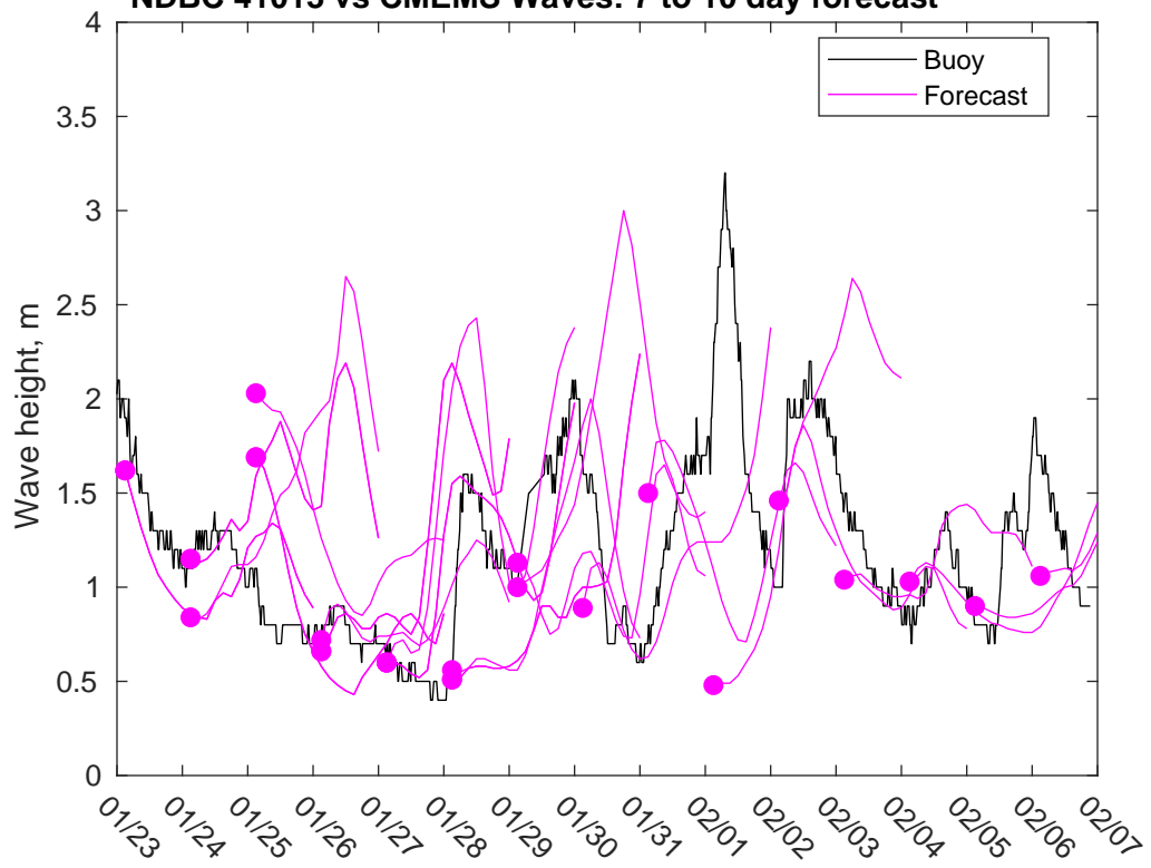
NDBC 41013 vs CMEMS Waves: 7 to 10 day forecast
