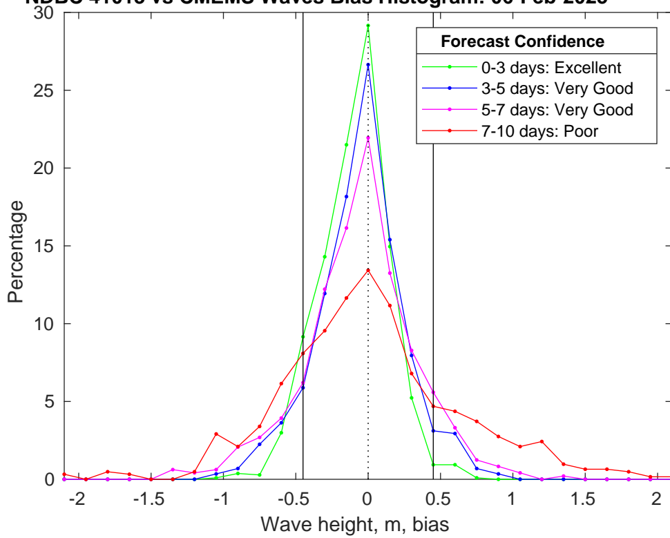
NDBC 41013 vs CMEMS Waves Bias Histogram: 06-Feb-2025
