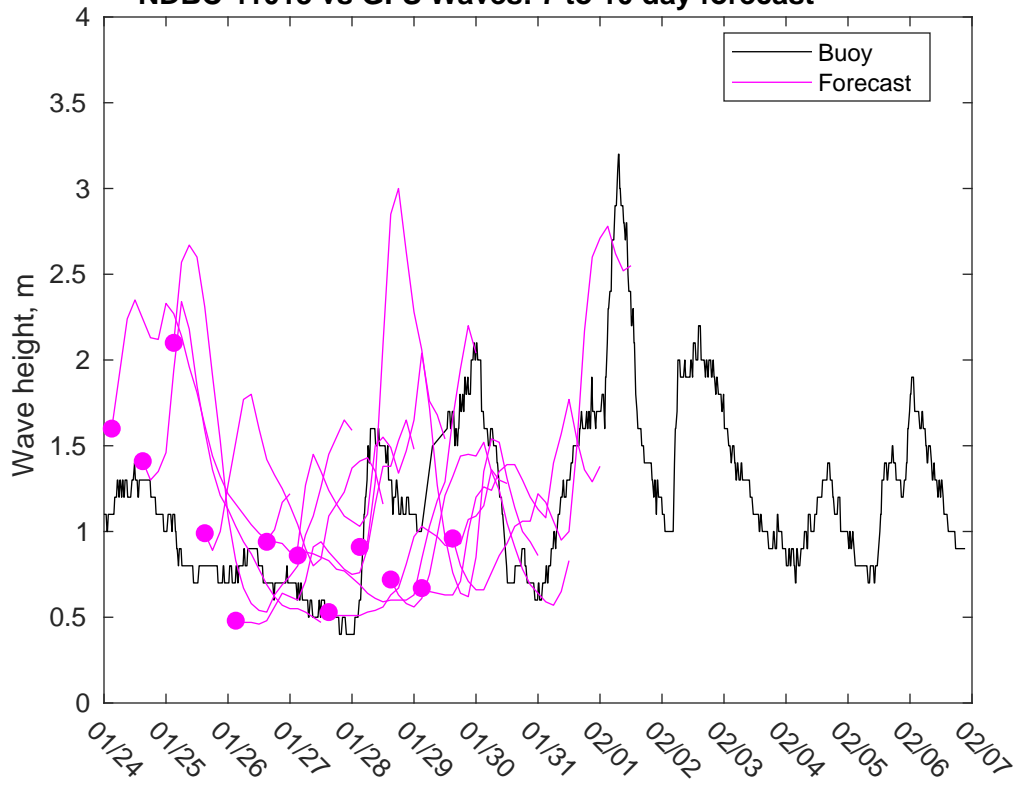
NDBC 41013 vs GFS Waves: 7 to 10 day forecast
