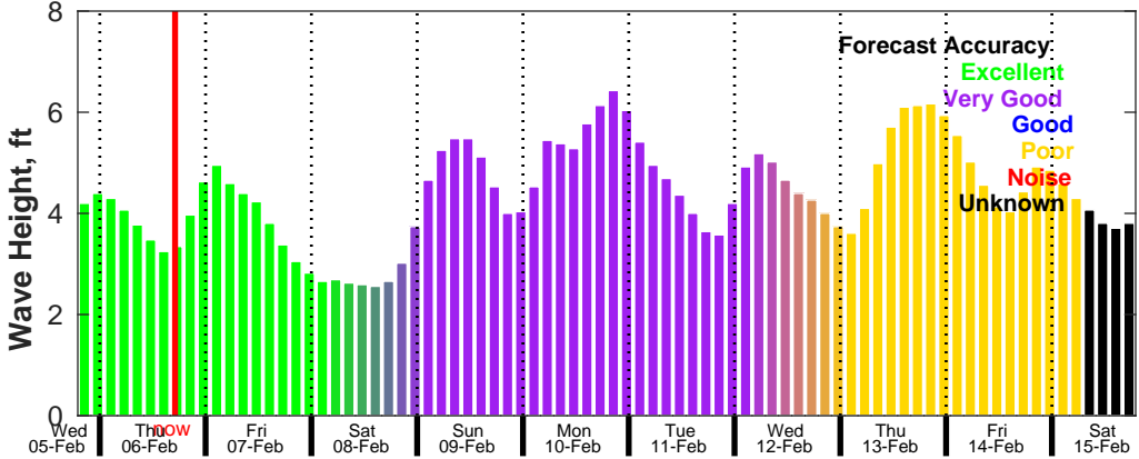
CMEMS Wave Forecast for NDBC 41013 from 05-Feb-2025 19:00:00 to 15-Feb-2025 19:00:00
