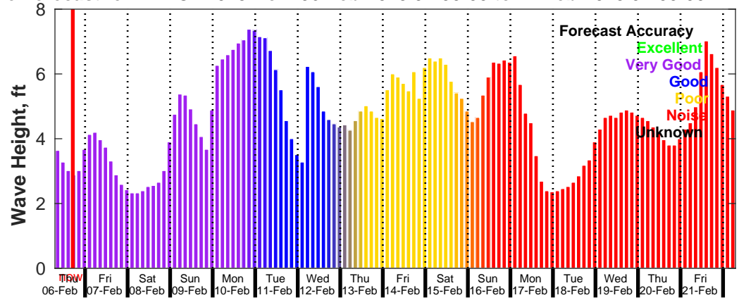
GFS Wave Forecast for NDBC 41013 from 06-Feb-2025 07:00:00 to 22-Feb-2025 07:00:00
