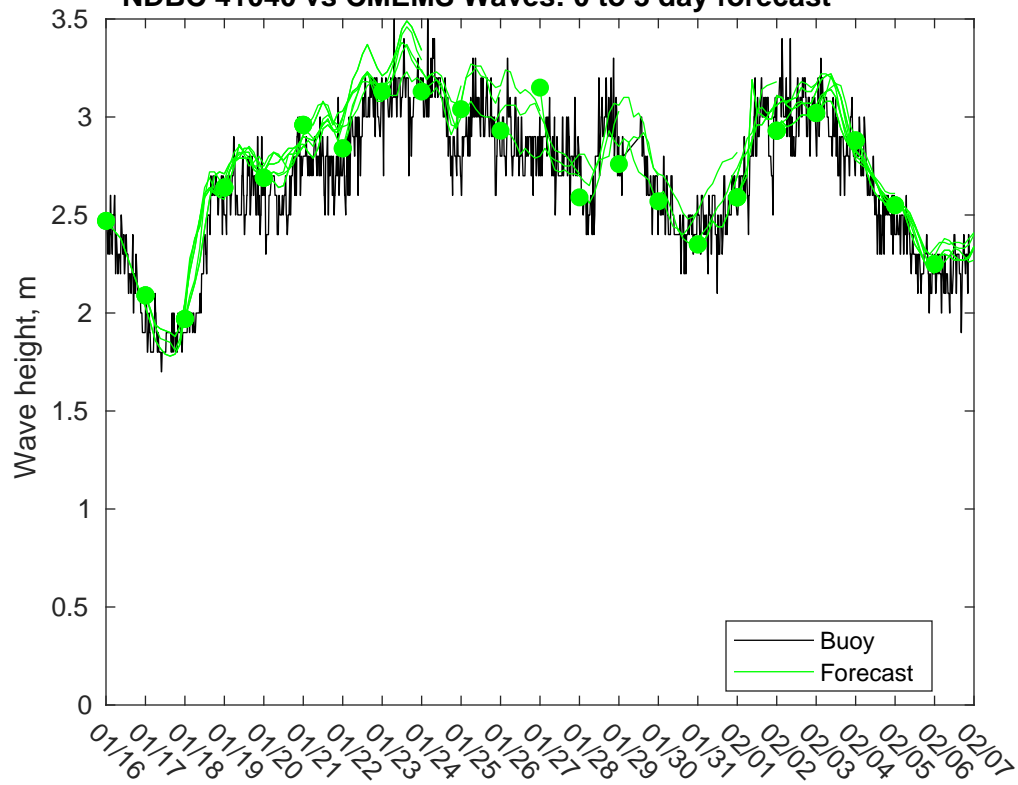
NDBC 41040 vs CMEMS Waves: 0 to 3 day forecast
