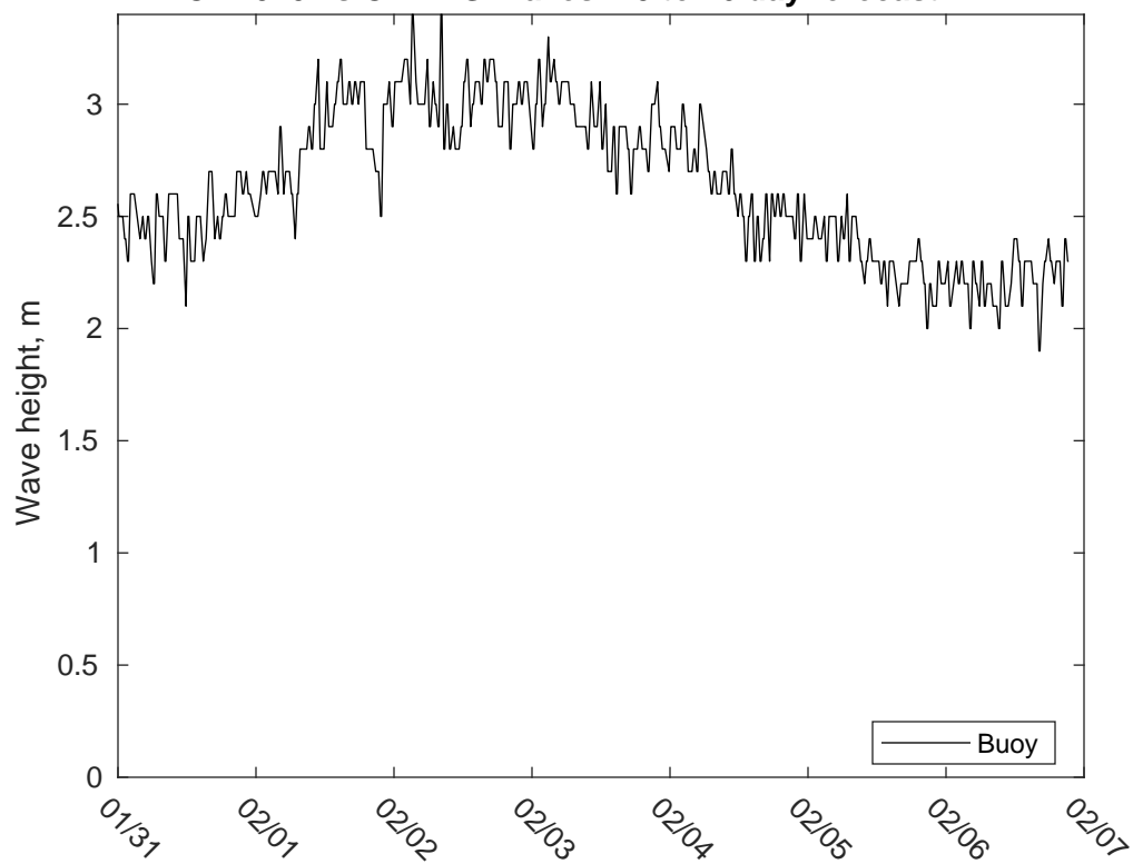
NDBC 41040 vs CMEMS Waves: 10 to 16 day forecast
