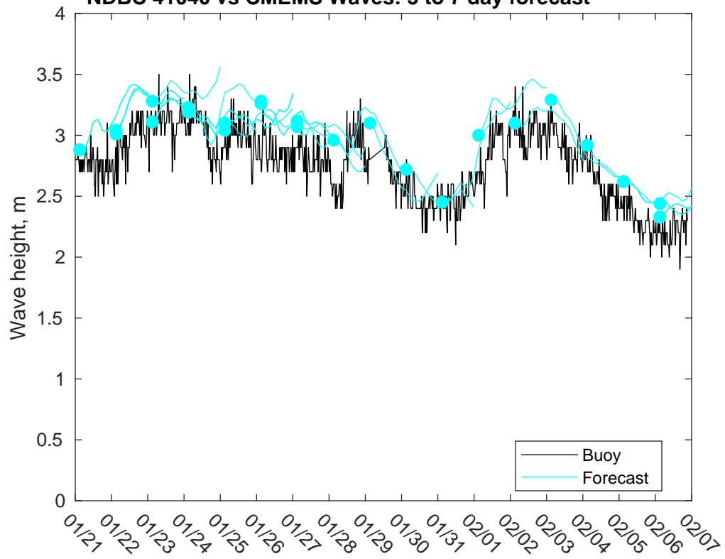
NDBC 41040 vs CMEMS Waves: 5 to 7 day forecast
