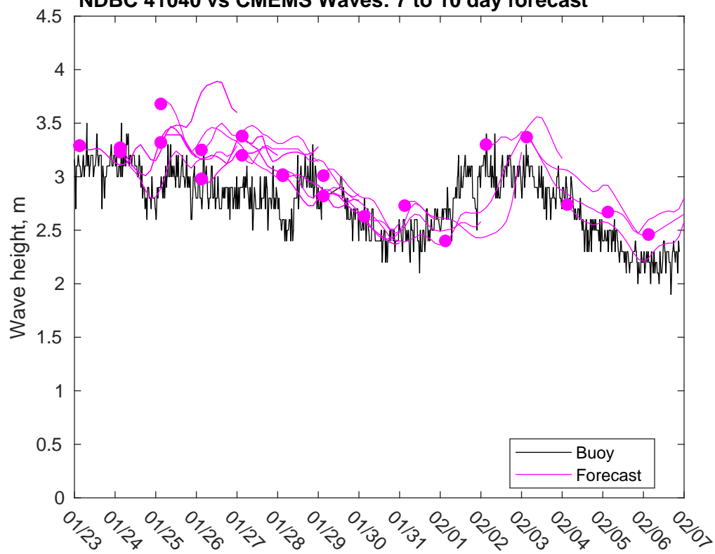
NDBC 41040 vs CMEMS Waves: 7 to 10 day forecast
