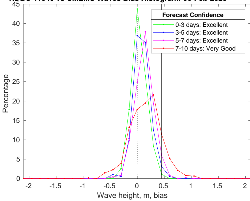
NDBC 41040 vs CMEMS Waves Bias Histogram: 06-Feb-2025
