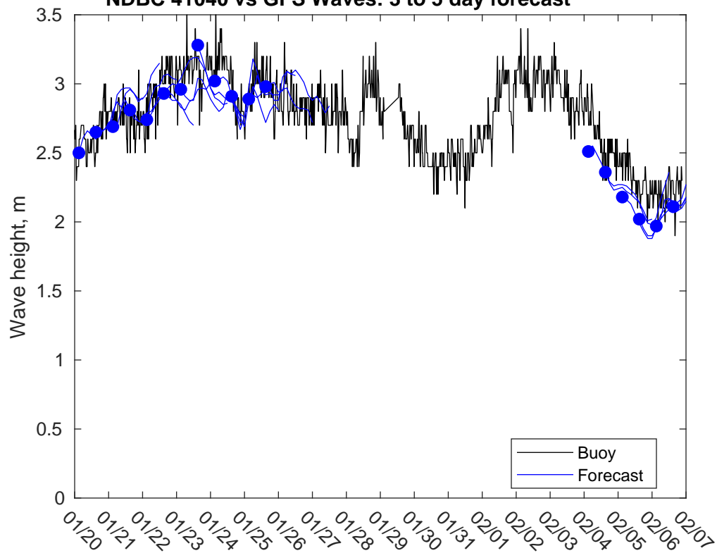
NDBC 41040 vs GFS Waves: 3 to 5 day forecast
