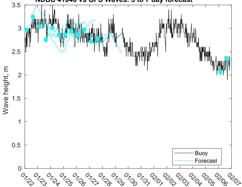
NDBC 41040 vs GFS Waves: 5 to 7 day forecast
