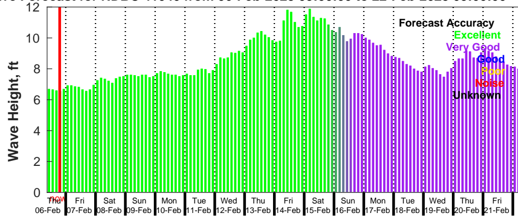
GFS Wave Forecast for NDBC 41040 from 06-Feb-2025 09:00:00 to 22-Feb-2025 09:00:00
