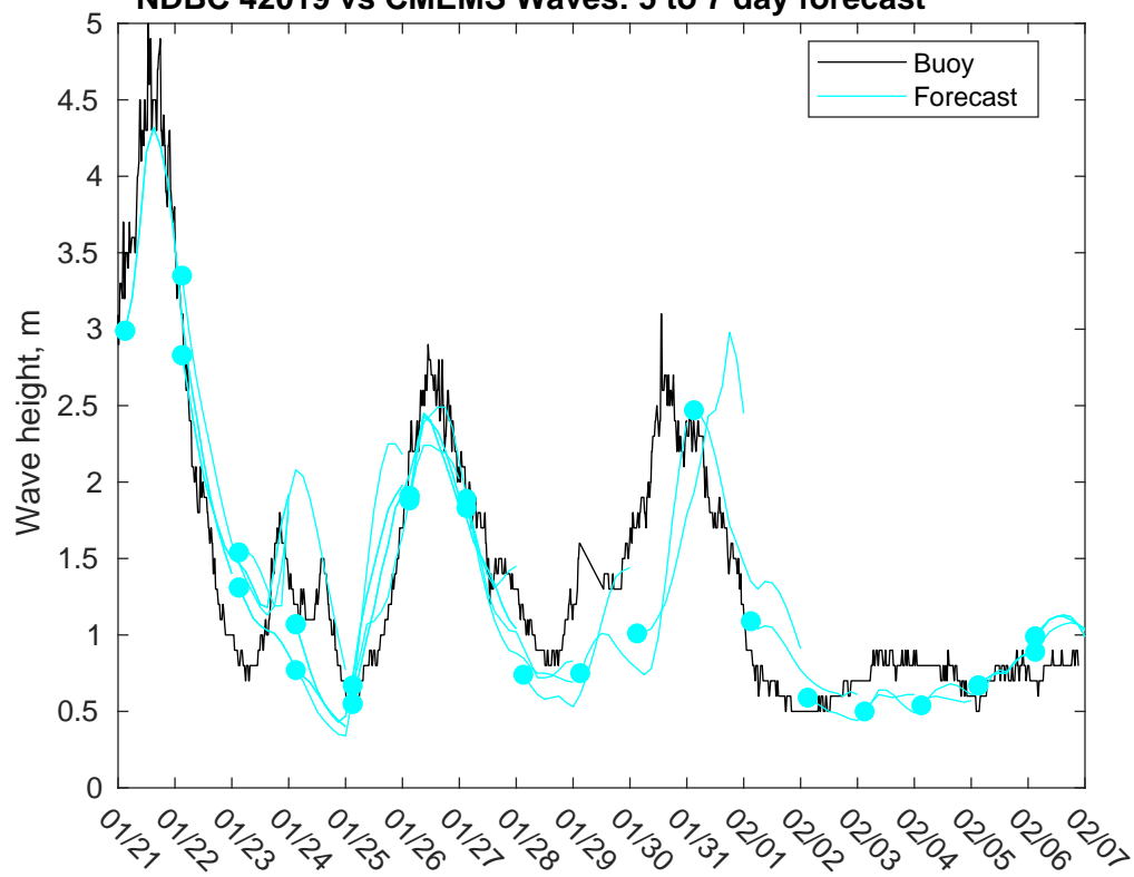
NDBC 42019 vs CMEMS Waves: 5 to 7 day forecast
