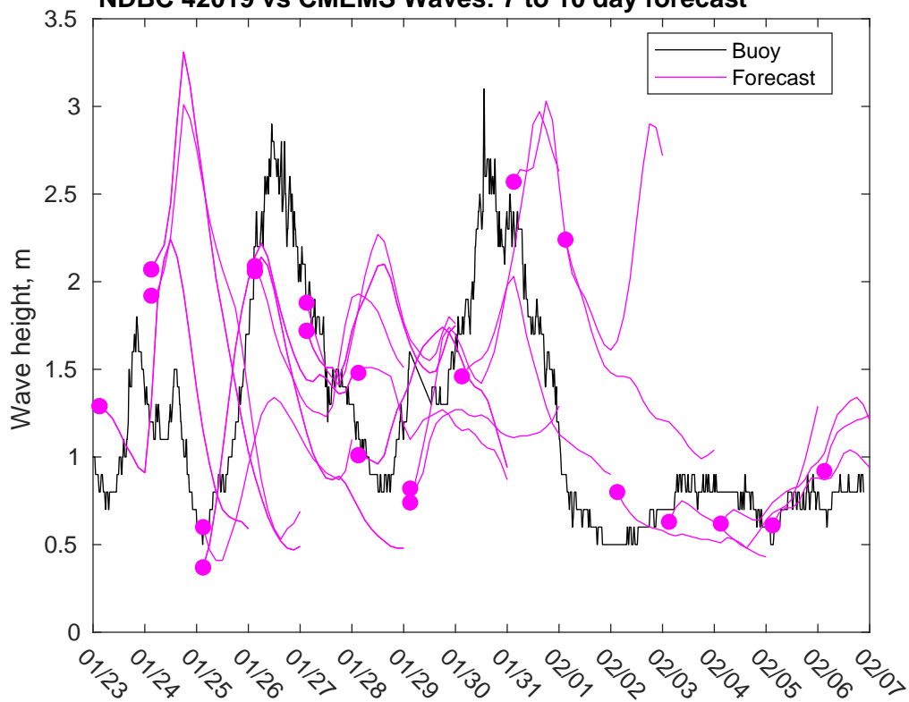
NDBC 42019 vs CMEMS Waves: 7 to 10 day forecast
