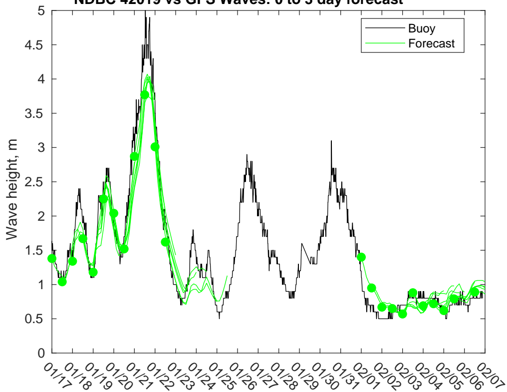
NDBC 42019 vs GFS Waves: 0 to 3 day forecast
