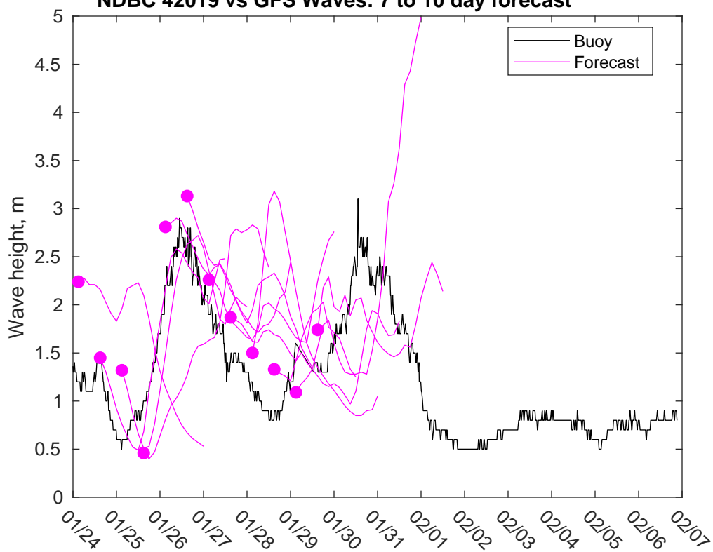
NDBC 42019 vs GFS Waves: 7 to 10 day forecast
