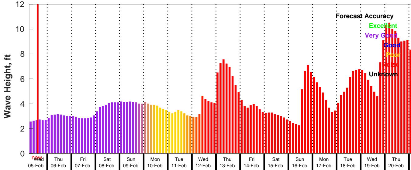
GFS Wave Forecast for NDBC 42019 from 05-Feb-2025 06:00:00 to 21-Feb-2025 06:00:00
