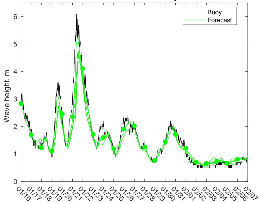
NDBC 42020 vs CMEMS Waves: 0 to 3 day forecast
