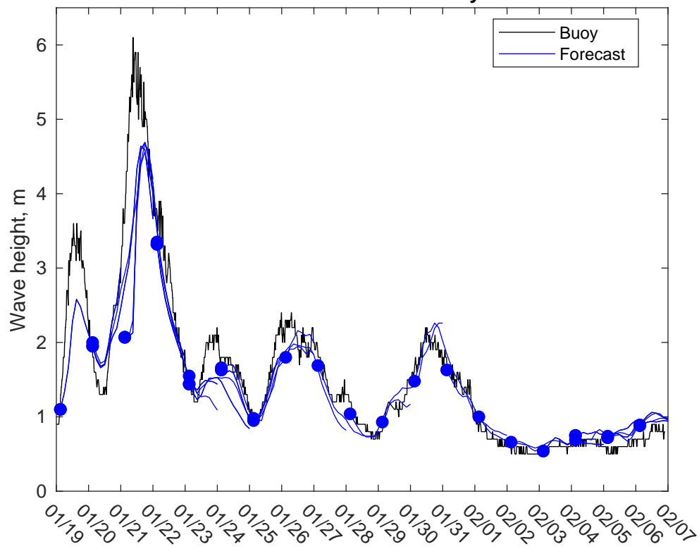
NDBC 42020 vs CMEMS Waves: 3 to 5 day forecast
