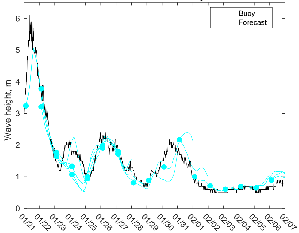
NDBC 42020 vs CMEMS Waves: 5 to 7 day forecast
