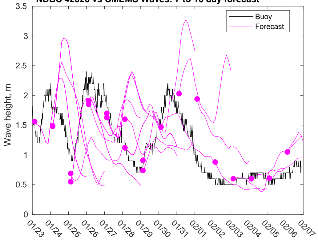
NDBC 42020 vs CMEMS Waves: 7 to 10 day forecast
