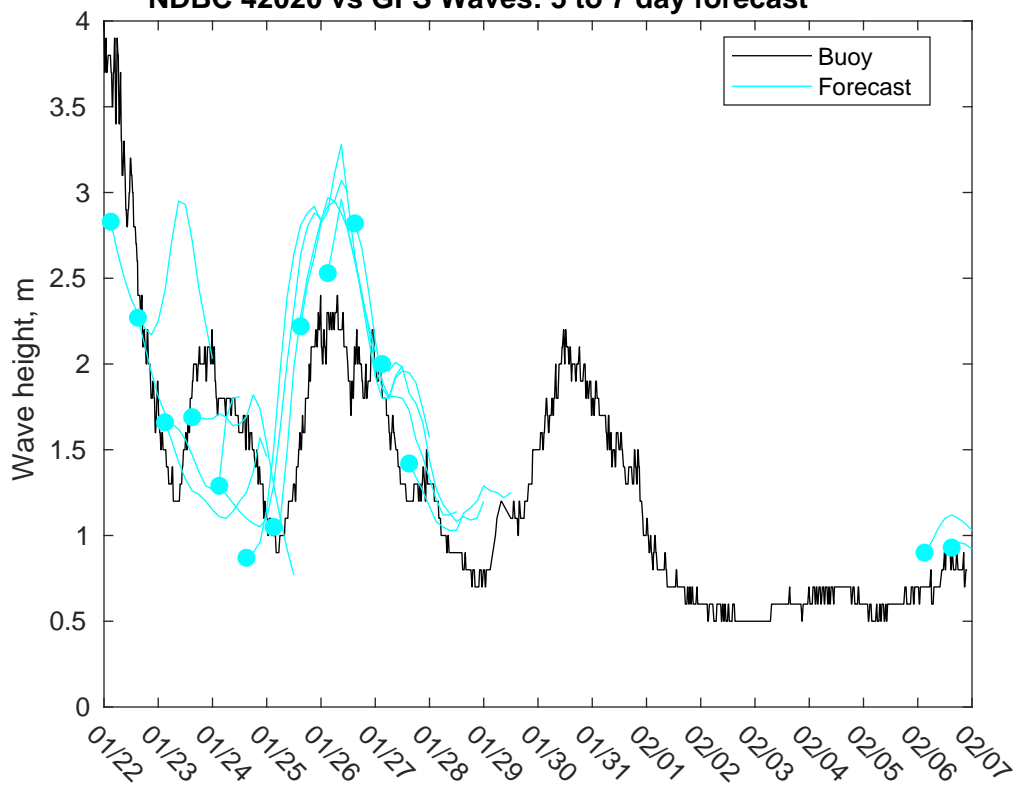
NDBC 42020 vs GFS Waves: 5 to 7 day forecast
