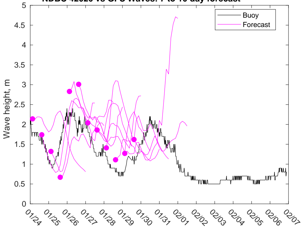
NDBC 42020 vs GFS Waves: 7 to 10 day forecast
