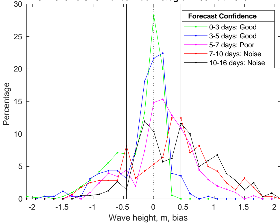
NDBC 42020 vs GFS Waves Bias Histogram: 06-Feb-2025
