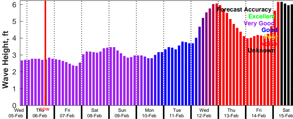
CMEMS Wave Forecast for NDBC 42020 from 05-Feb-2025 18:00:00 to 15-Feb-2025 18:00:00
