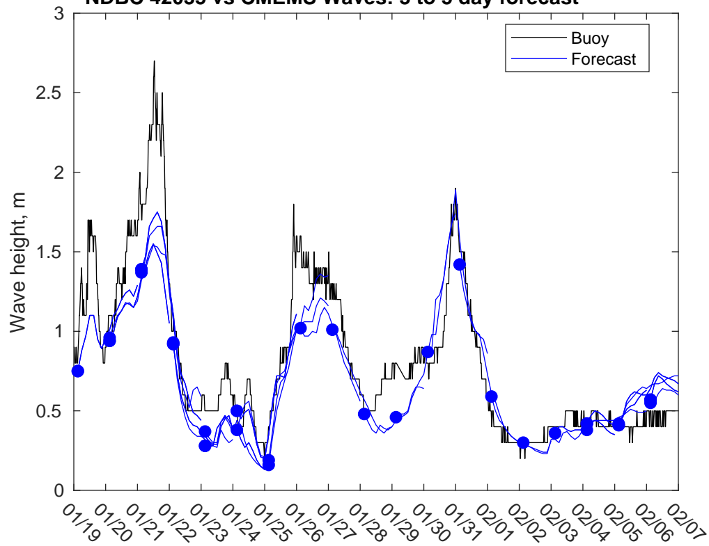
NDBC 42035 vs CMEMS Waves: 3 to 5 day forecast
