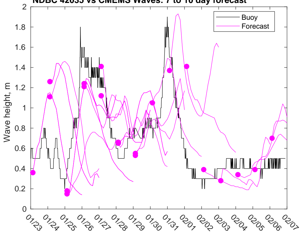
NDBC 42035 vs CMEMS Waves: 7 to 10 day forecast
