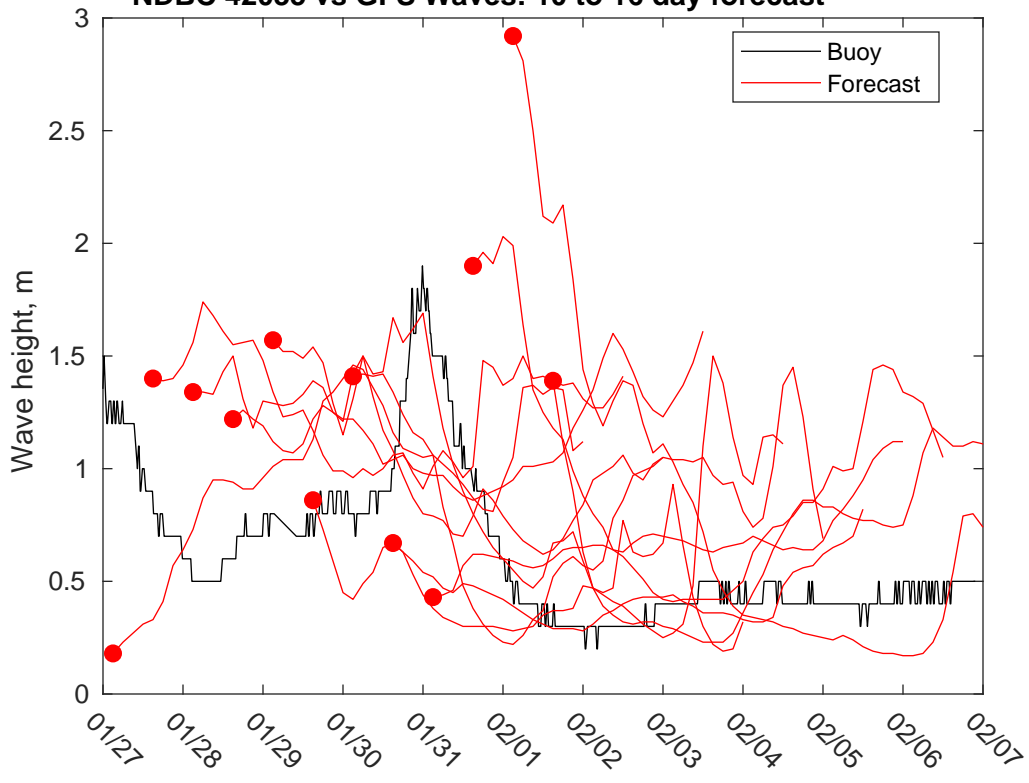
NDBC 42035 vs GFS Waves: 10 to 16 day forecast
