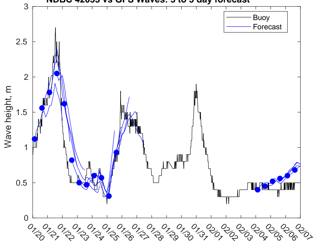
NDBC 42035 vs GFS Waves: 3 to 5 day forecast
