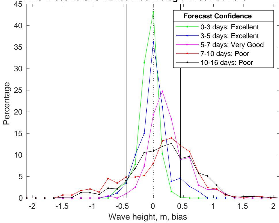
NDBC 42035 vs GFS Waves Bias Histogram: 06-Feb-2025
