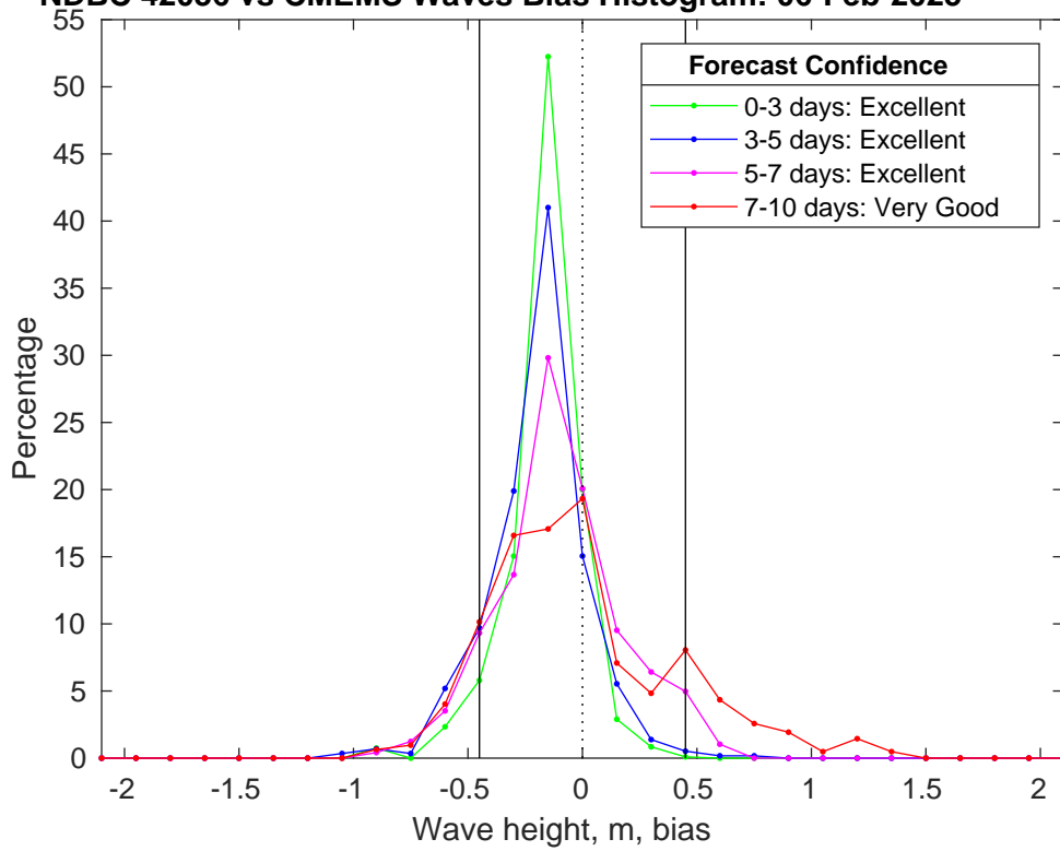
NDBC 42036 vs CMEMS Waves Bias Histogram: 06-Feb-2025
