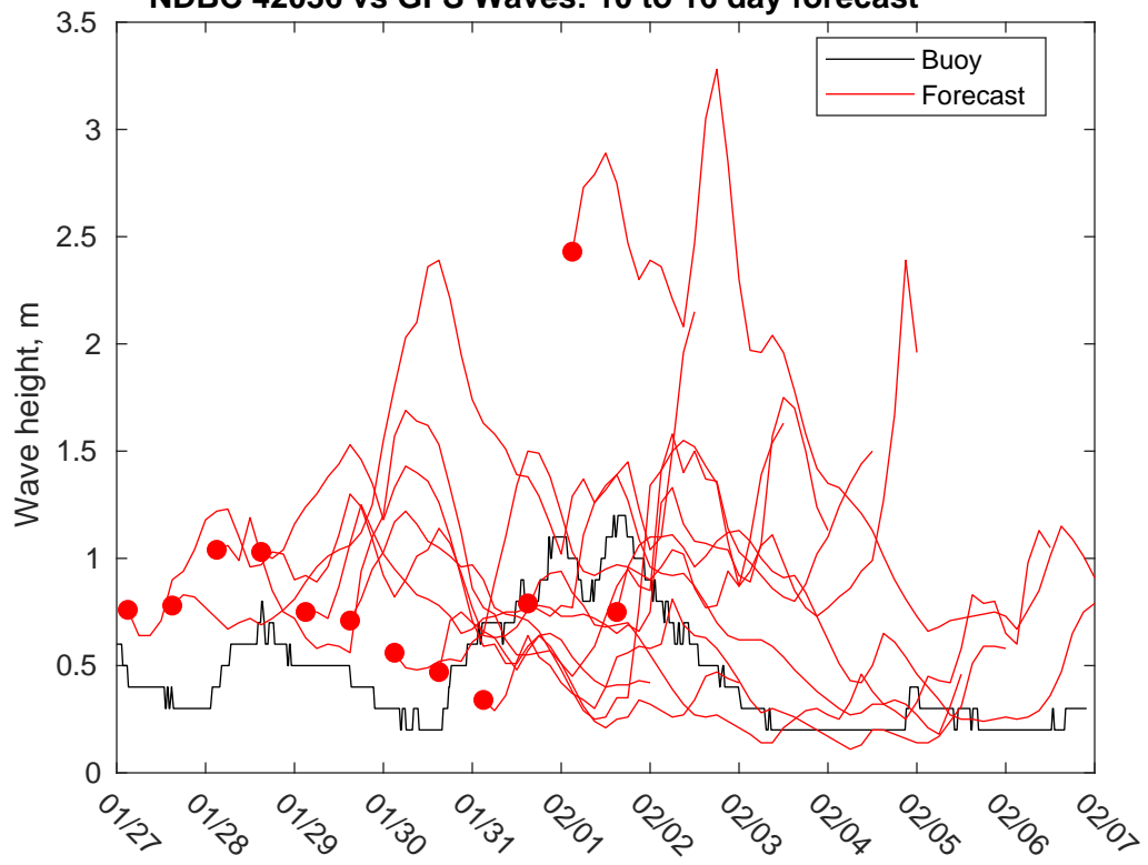
NDBC 42036 vs GFS Waves: 10 to 16 day forecast
